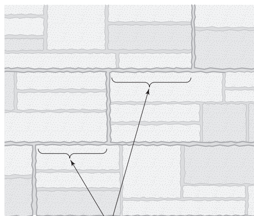
Minimum of 8" stagger between courses
