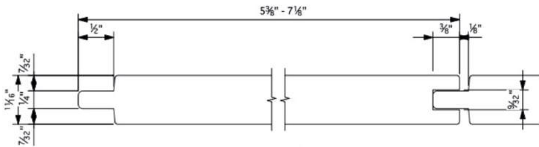
Elite Finline ( \frac{1}{8} th Gap) Paneling
